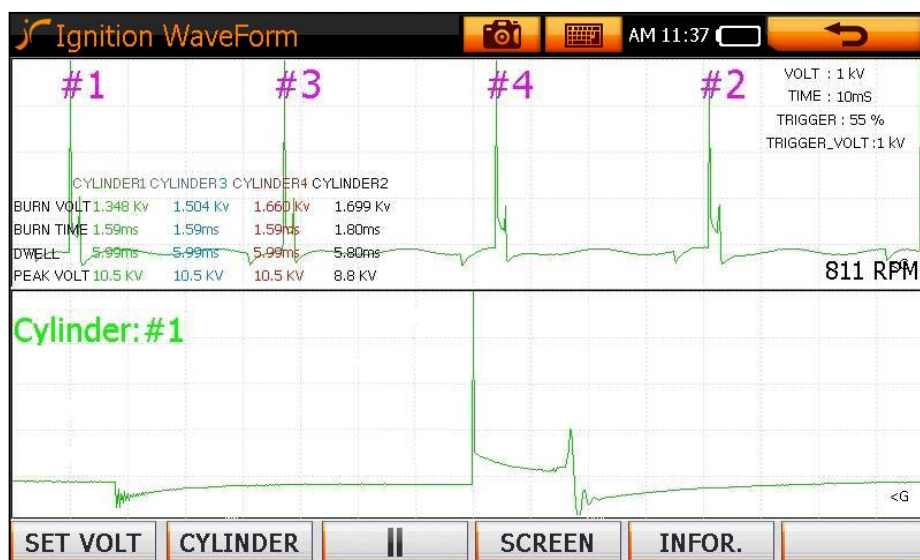
Fig. XIV-32 Measurement of Ignition Waveform
