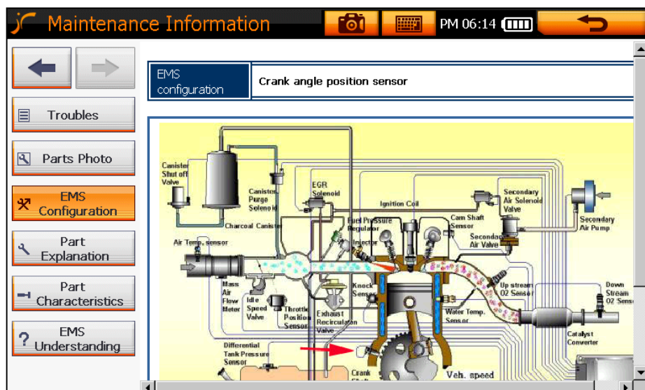
Fig. XI-5 EMS Simple Diagram
